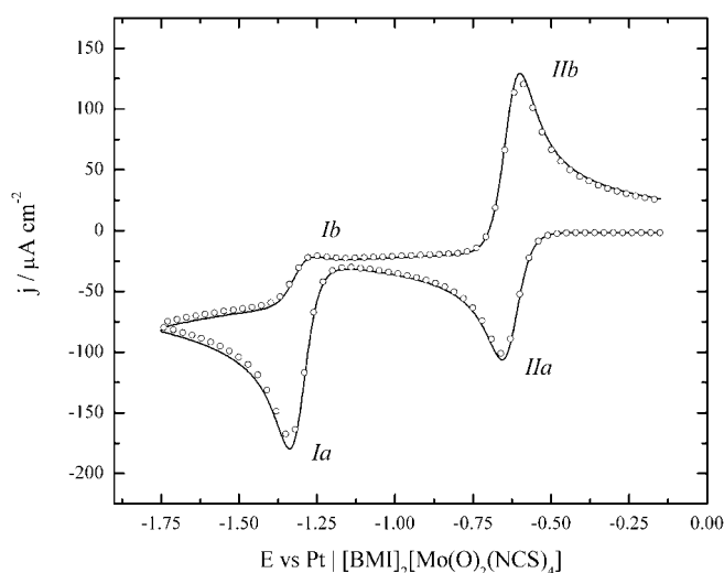
Figure 1. Cyclic voltammogram of neat 2 at a Pt electrode [12] and a scan rate \nu = 10 \text{ mV s}^{-1} . Dots: numerical simulation of an ECE mechanism. Potentials are referred to a pseudo-reference Pt electrode.
